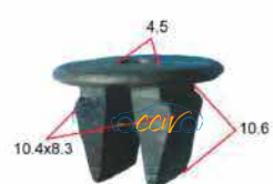
Black Plastic Screw Grommets 25pcs
