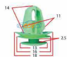
Hyundai Trim Clips 25pcs
