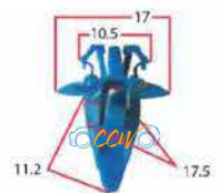
Toyota Blue Body Flare Clips 25pcs
