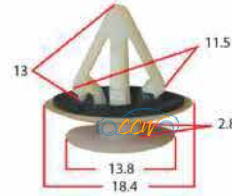
Mazda Trim Clips 25pcs
