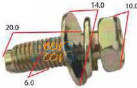
8.8 M6 10mm Head-Bolt With Spring Washer 25pcs
