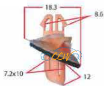
Toyota Salmon Body Flare Clips 25pcs
