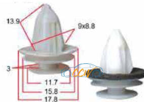
Universal Trim Clips 25pcs
