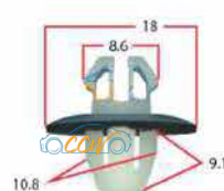
Toyota White Body Flare Clips 25pcs
