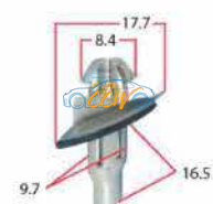
Toyota Grey Body Flare Clips 25pcs
