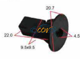
Toyota Inner Guard Grommets 25pcs
