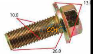
8.8-M10 Flange Bolts 25pcs
