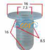
Trim Mould Clips 25pcs
