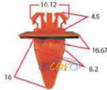
Toyota Red Body Flare Clips 25pcs
