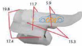
Toyota Body Clips 25pcs
