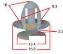
Liveco Body Trim & Mould Clips 25pcs
