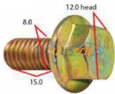
8.8 M8 12mm Head Flange Bolts 25pcs
